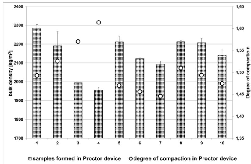
Fig. 3. Density and degree of compaction of concrete samples
