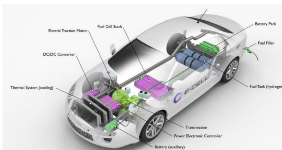
Figure 1. Fuel cell vehicle with on-board storage [29].
