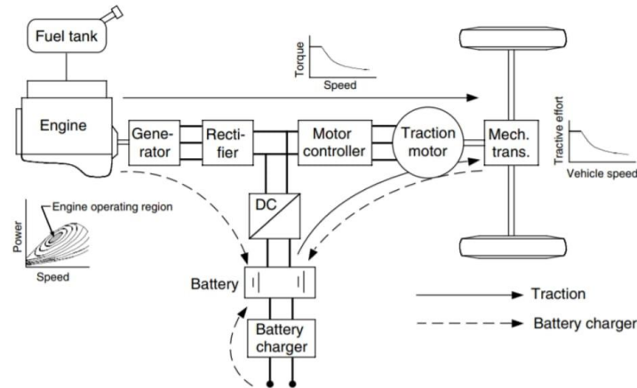
Figure 6. Series hybrid configuration [35].
