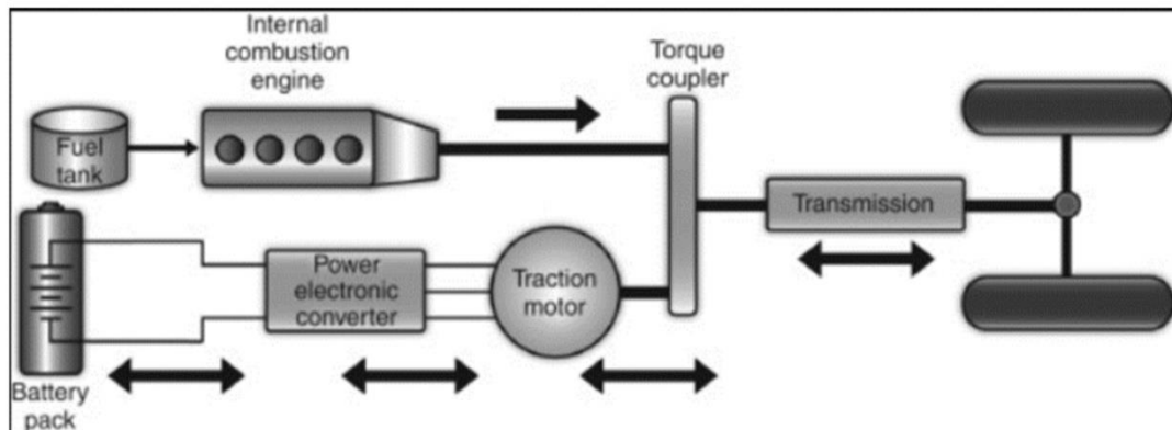
Figure 5. Parallel hybrid configuration [69].
