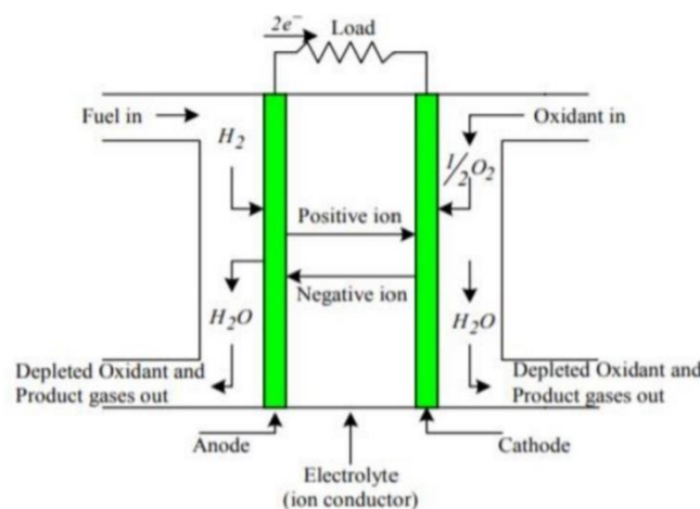
Figure 2. Fuel cell operation diagram [38].
