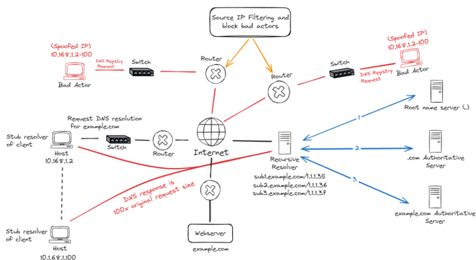
Figure 5: A Network Diagram Showing Where Bad Actors Are Blocked Prior To Reaching The DNS
